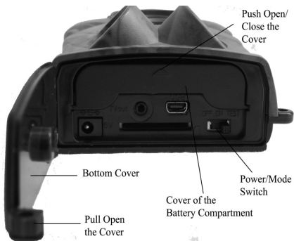
Figure 1.2: Bottom View of Ltl-5310M
